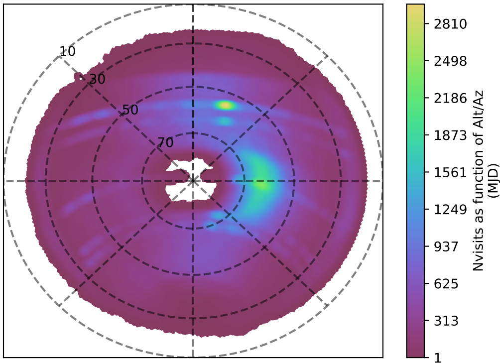
ddf_acor_sf15_lsf40_lsr50_v3.4_10yrs z band: Nvisits as function of Alt/Az
