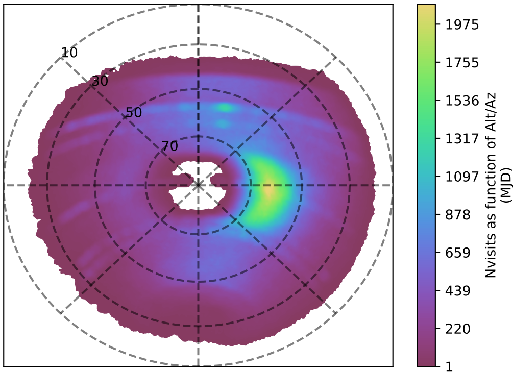
ddf_acor_sf15_lsf40_lsr50_v3.4_10yrs y band: Nvisits as function of Alt/Az
