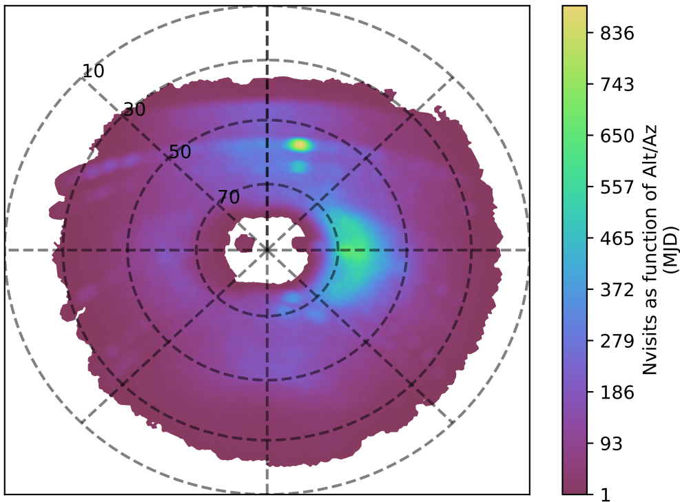
ddf_acor_sf15_lsf40_lsr50_v3.4_10yrs u band: Nvisits as function of Alt/Az
