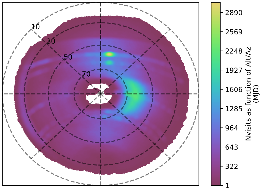
ddf_acor_sf15_lsf40_lsr50_v3.4_10yrs r band: Nvisits as function of Alt/Az
