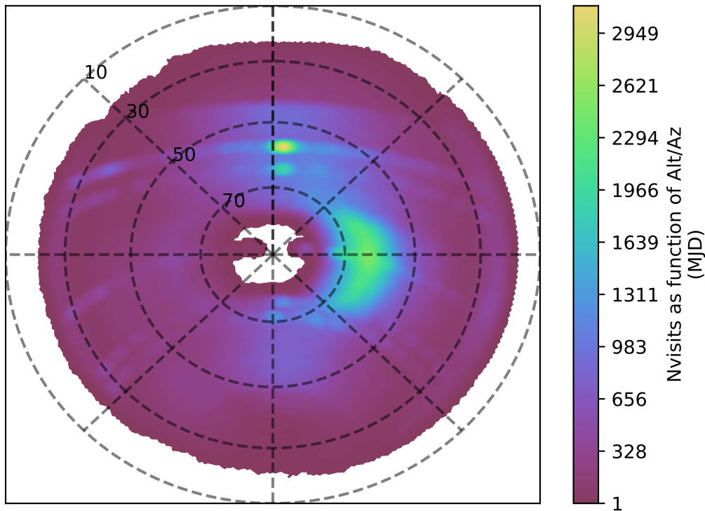
ddf_acor_sf15_lsf40_lsr50_v3.4_10yrs i band: Nvisits as function of Alt/Az
