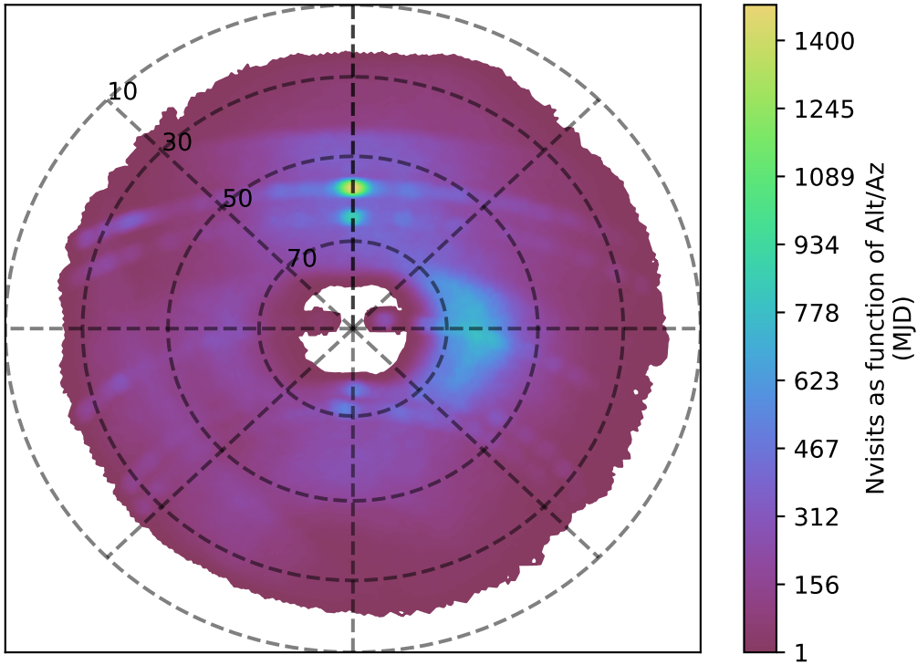
ddf_acor_sf15_lsf40_lsr50_v3.4_10yrs g band: Nvisits as function of Alt/Az
