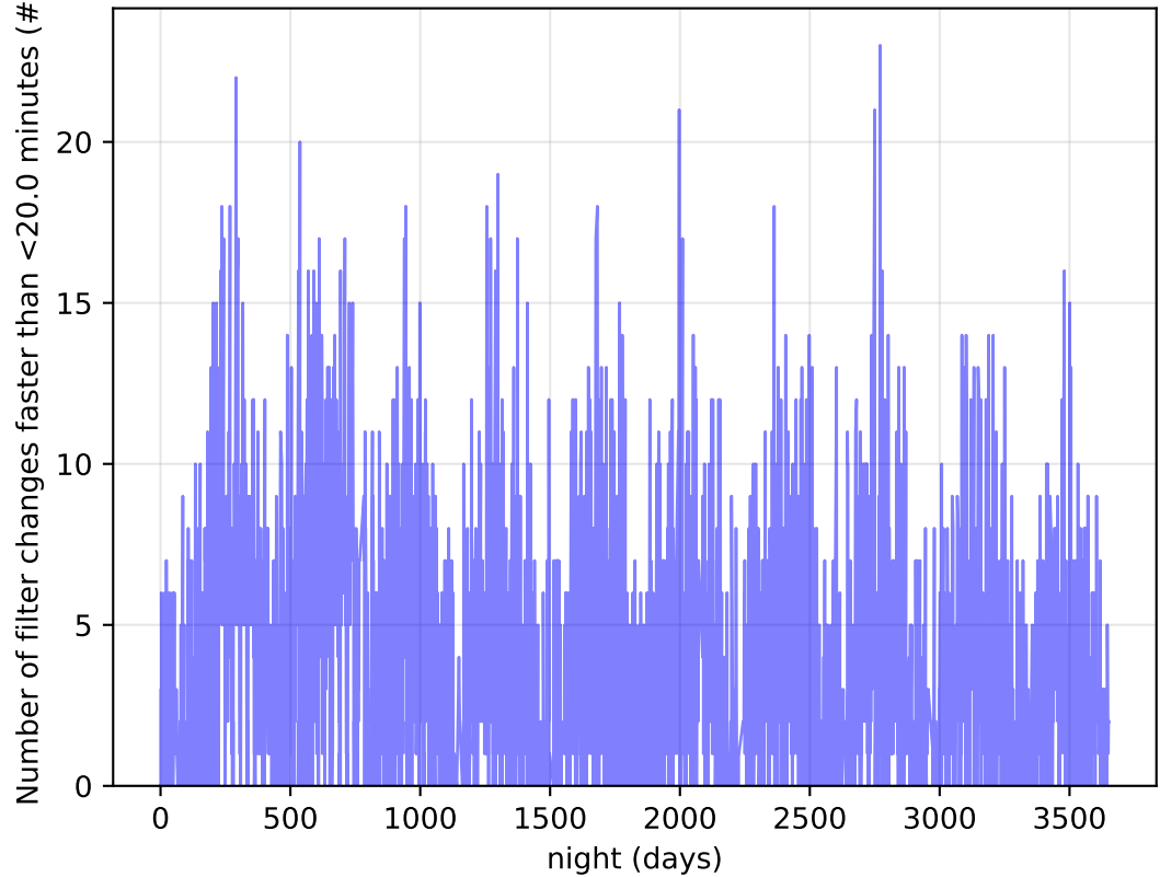
ddf_acor_sf15_Isf40_Isr50_v3.4_10yrs Per Night: Number of filter changes faster than <20.0 minutes
