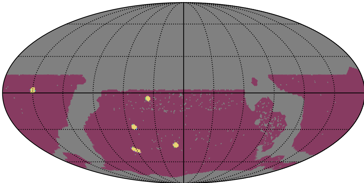
ddf_acor_sf15_lsf40_lsr50_v3.4_10yrs WFD: NumberOfQuickRevisits
