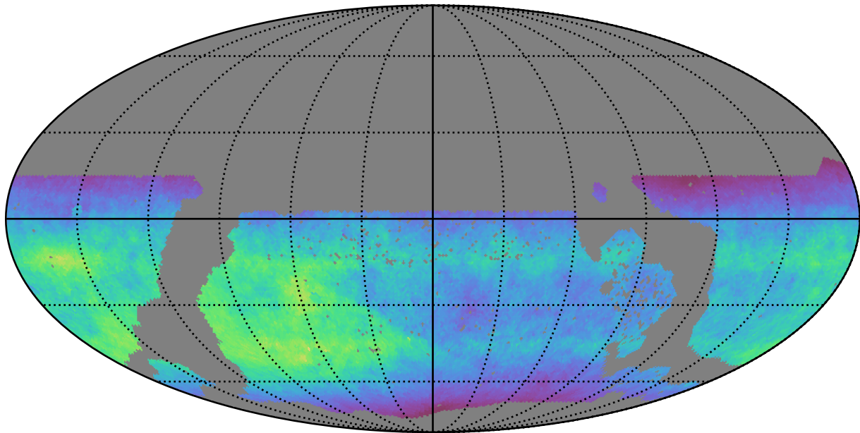
ddf_acor_sf15_lsf40_lsr50_v3.4_10yrs WFD i band: Normalized Teff
