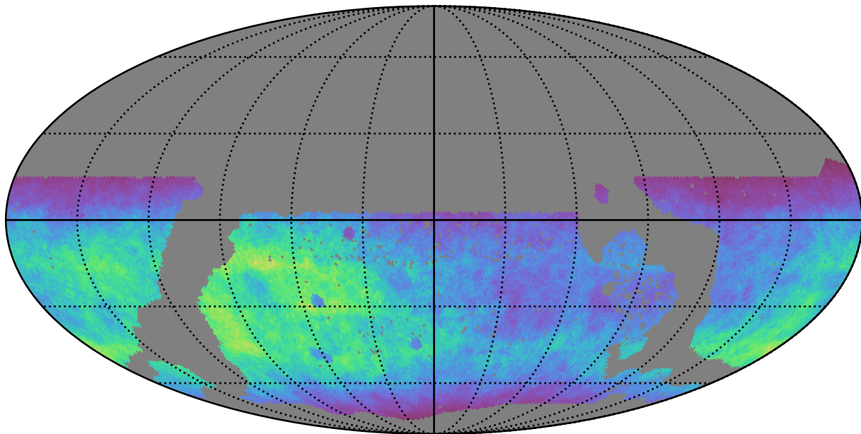
ddf_acor_sf15_lsf40_lsr50_v3.4_10yrs WFD g band: Normalized Teff
