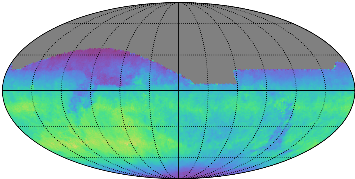
ddf_acor_sf15_lsf40_lsr50_v3.4_10yrs All sky z band: Normalized Teff
