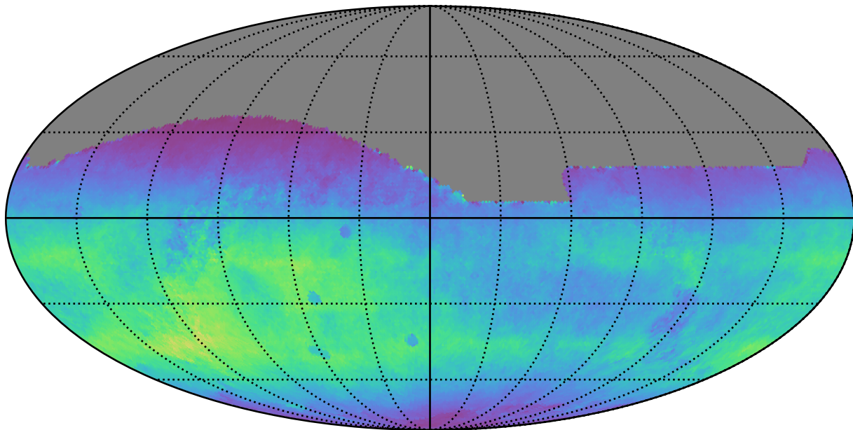
ddf_acor_sf15_lsf40_lsr50_v3.4_10yrs All sky r band: Normalized Teff
