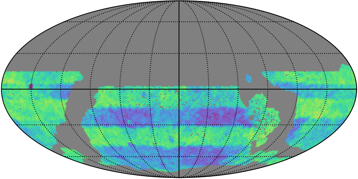
ddf_acor_sf15_lsf40_lsr50_v3.4_10yrs WFD: Normalized Proper Motion Uncert @ 24.0
