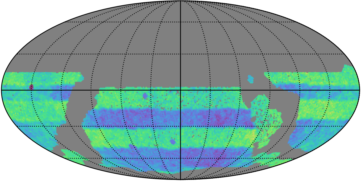
ddf_acor_sf15_lsf40_lsr50_v3.4_10yrs WFD: Normalized Proper Motion Uncert @ 20.5
