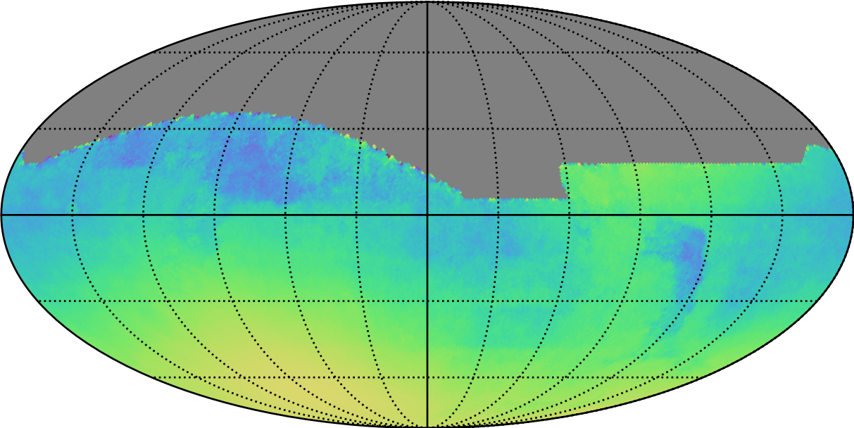
ddf_acor_sf15_lsf40_lsr50_v3.4_10yrs All sky: Normalized Parallax Uncert @ 24.0
