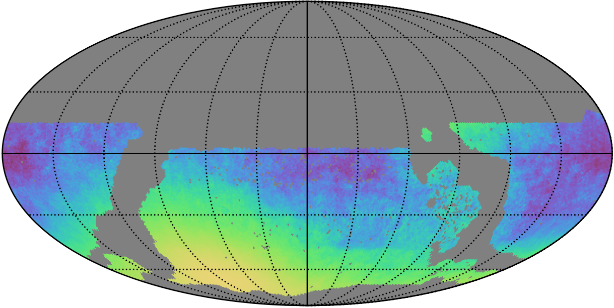
ddf_acor_sf15_lsf40_lsr50_v3.4_10yrs WFD y band only: Normalized Parallax Uncert @ 21.3
