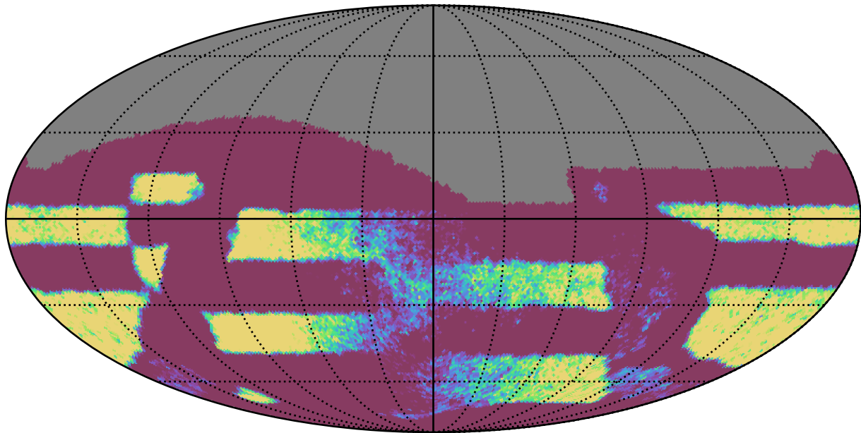
ddf_acor_sf15_lsf40_lsr50_v3.4_10yrs Yr 3-4 all bands: NVisits
