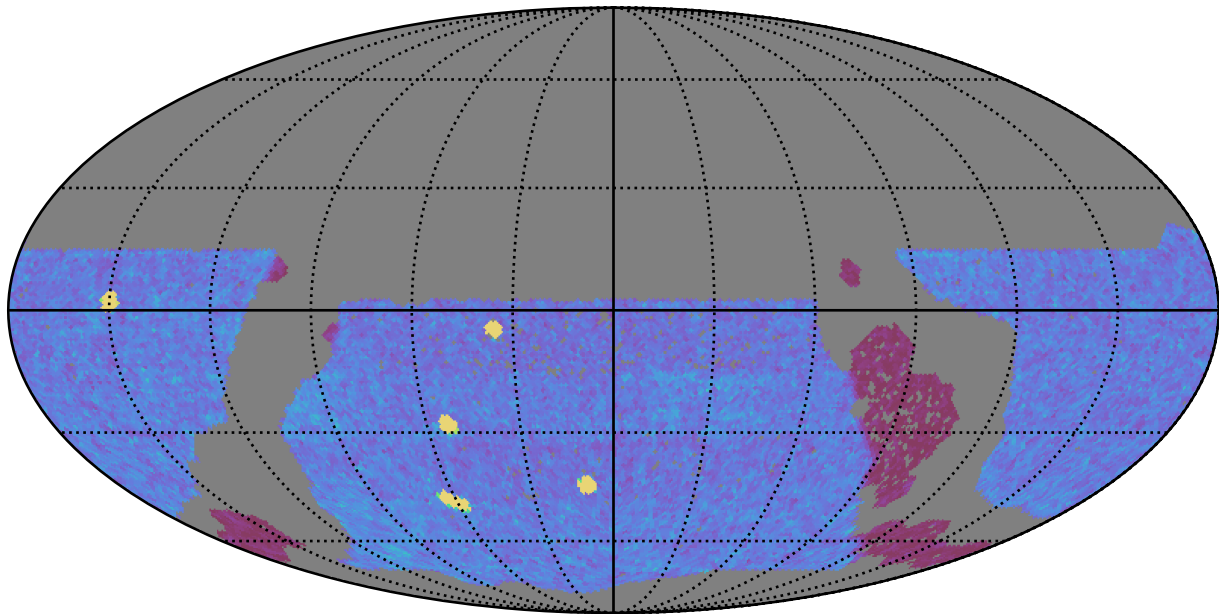
ddf_acor_sf15_lsf40_lsr50_v3.4_10yrs WFD y band: NVisits
