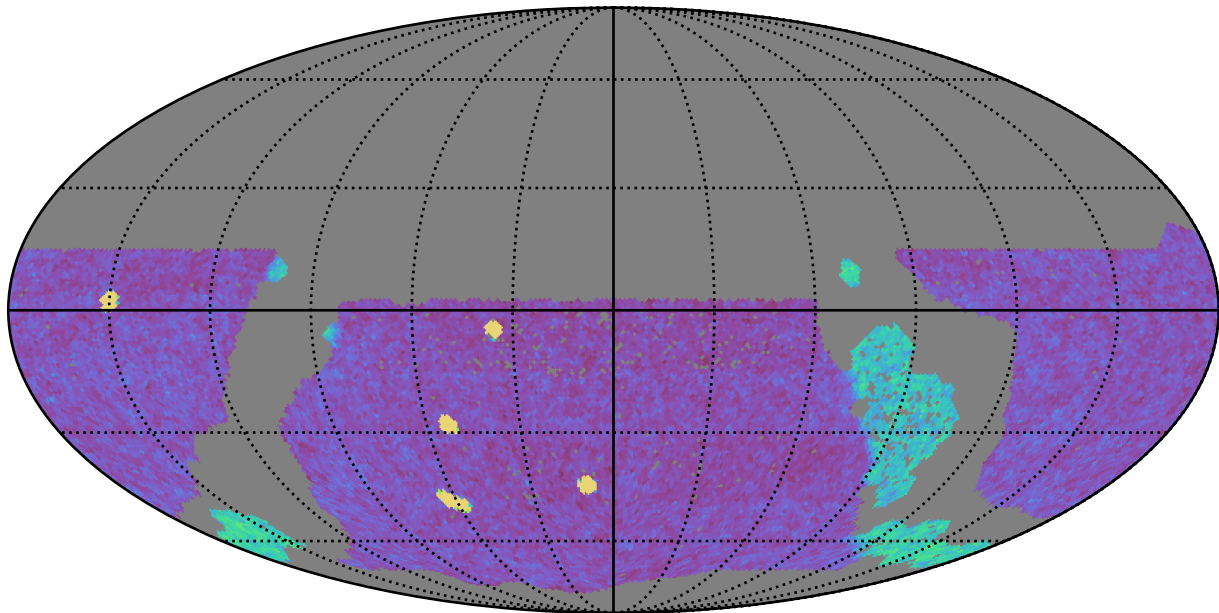
ddf_acor_sf15_lsf40_lsr50_v3.4_10yrs WFD g band: NVisits
