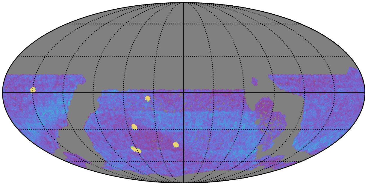
ddf_acor_sf15_lsf40_lsr50_v3.4_10yrs WFD all bands: NVisits
