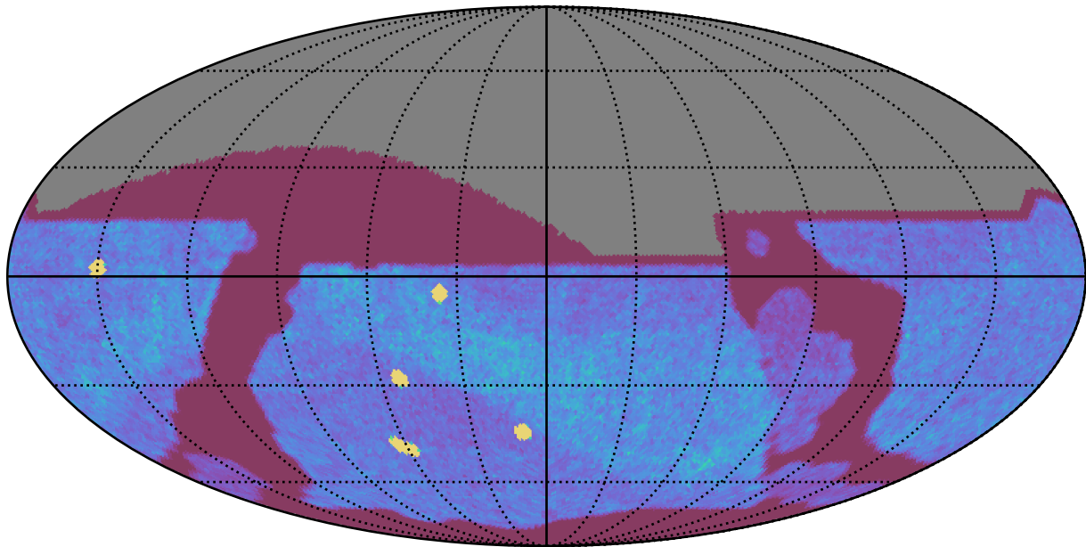
ddf_acor_sf15_lsf40_lsr50_v3.4_10yrs All sky z band: NVisits
