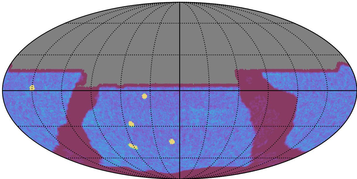
ddf_acor_sf15_lsf40_lsr50_v3.4_10yrs All sky y band: NVisits
