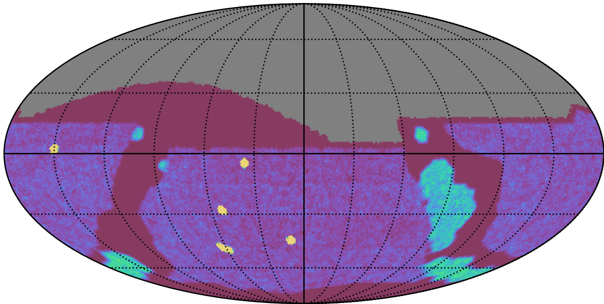
ddf_acor_sf15_lsf40_lsr50_v3.4_10yrs All sky g band: NVisits
