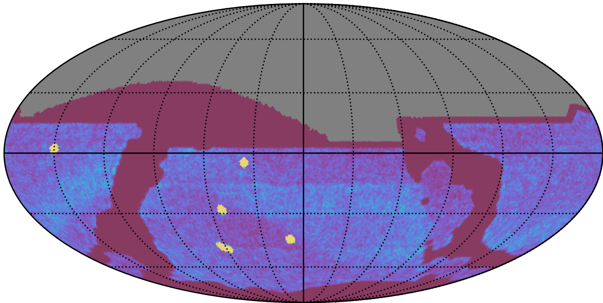
ddf_acor_sf15_lsf40_lsr50_v3.4_10yrs All sky all bands: NVisits
