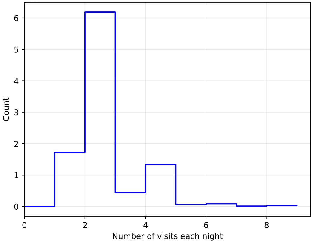
ddf_acor_sf15_lsf40_lsr50_v3.4_10yrs All sky: NVisitsPerNight 1e6
