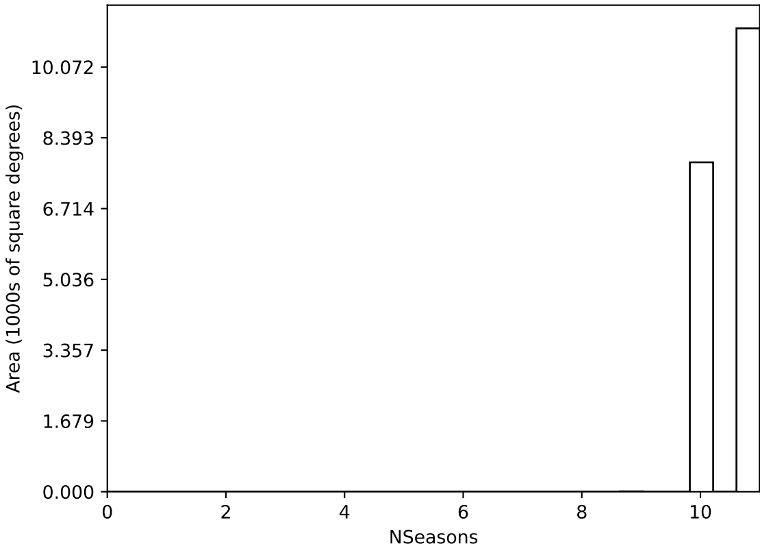
ddf_acor_sf15_lsf40_lsr50_v3.4_10yrs WFD all bands: NSeasons
