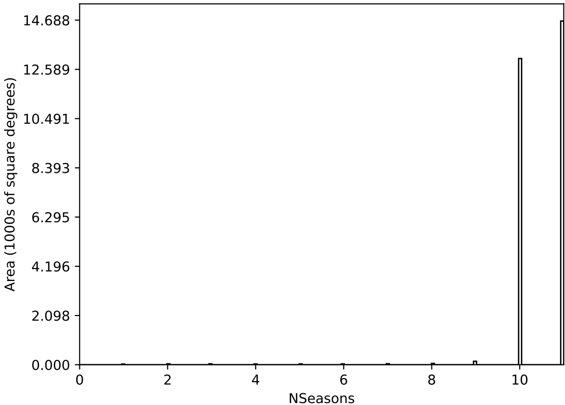
ddf_acor_sf15_lsf40_lsr50_v3.4_10yrs All sky all bands: NSeasons
