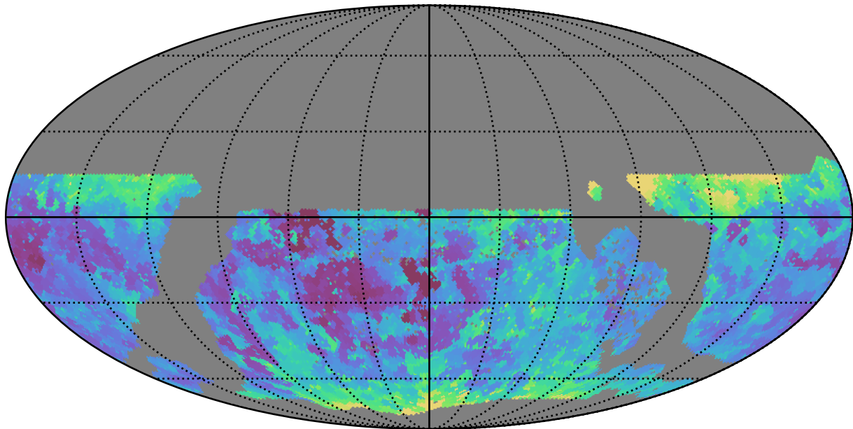
ddf_acor_sf15_lsf40_lsr50_v3.4_10yrs WFD g band: Min seeingEff
