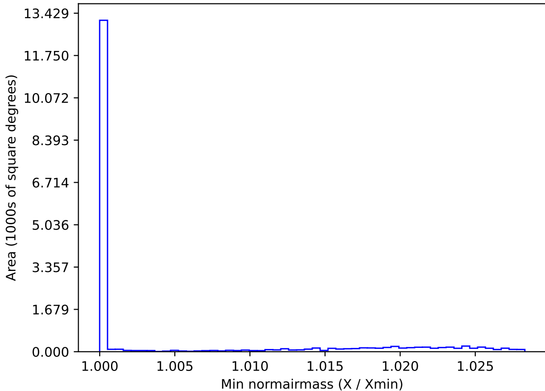
ddf_acor_sf15_lsf40_lsr50_v3.4_10yrs WFD all bands: Min normairmass
