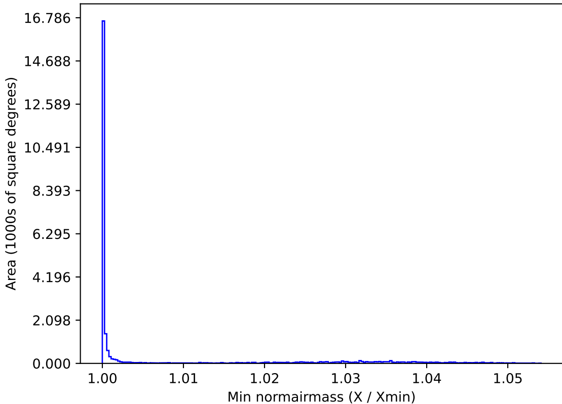
ddf_acor_sf15_lsf40_lsr50_v3.4_10yrs All sky g band: Min normairmass
