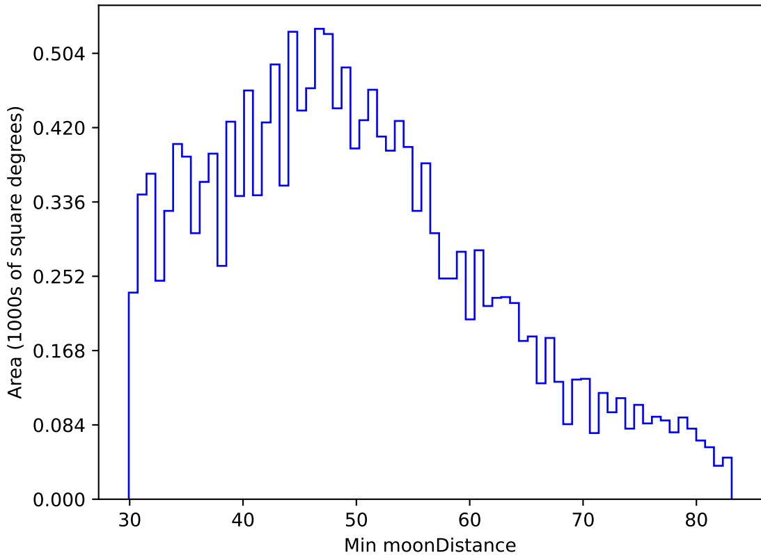
ddf_acor_sf15_lsf40_lsr50_v3.4_10yrs WFD u band: Min moonDistance
