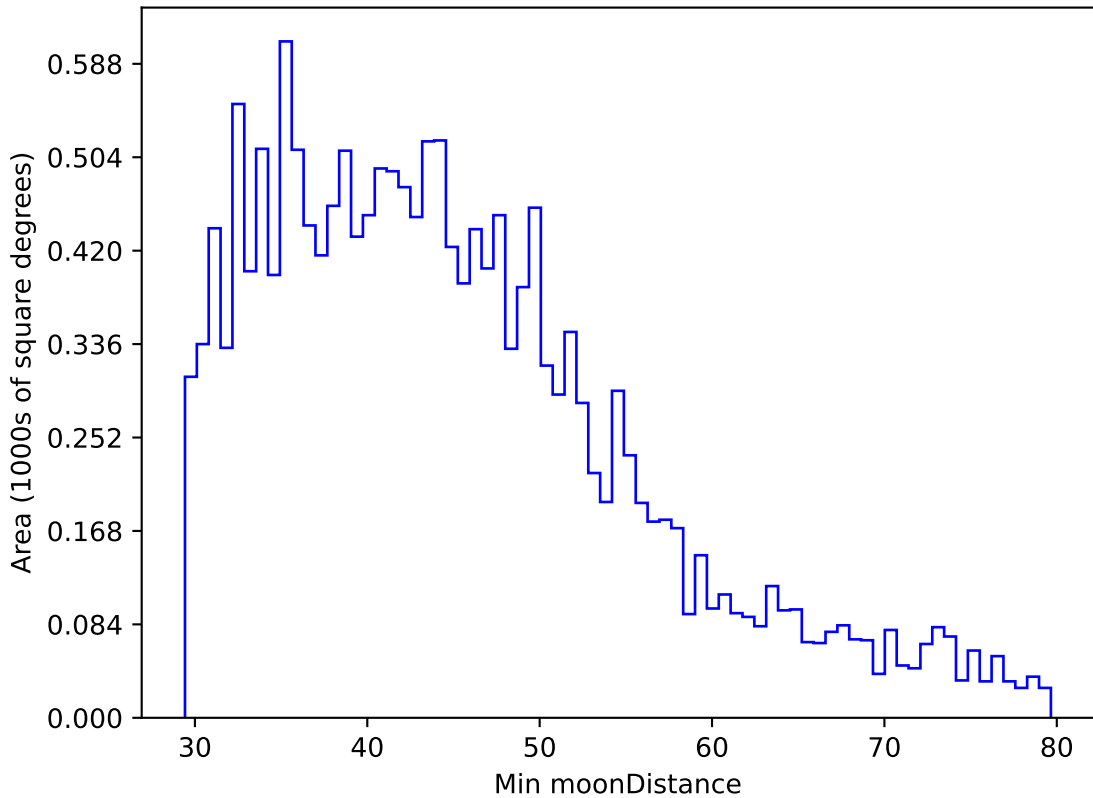
ddf_acor_sf15_lsf40_lsr50_v3.4_10yrs WFD g band: Min moonDistance
