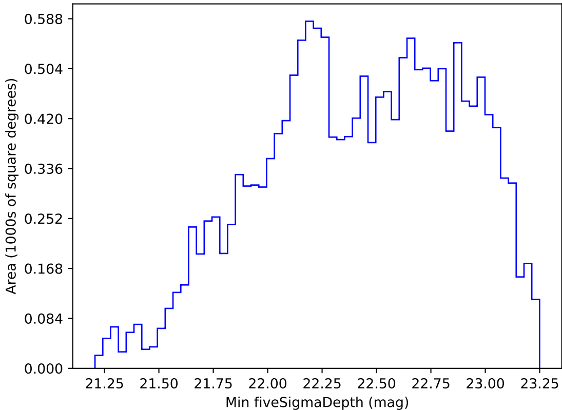
ddf_acor_sf15_ls40_lsr50_v3.4_10yrs WFD r band: Min fiveSigmaDepth
