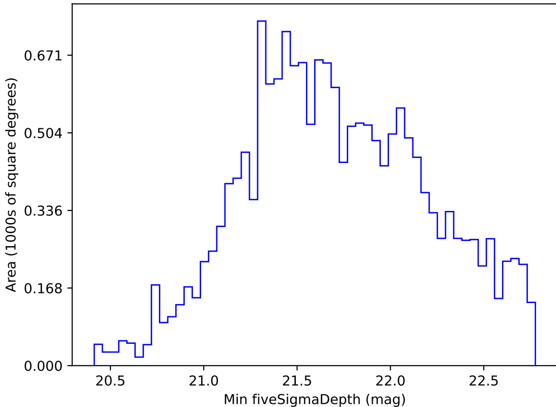
ddf_acor_sf15_lsf40_lsr50_v3.4_10yrs WFD i band: Min fiveSigmaDepth
