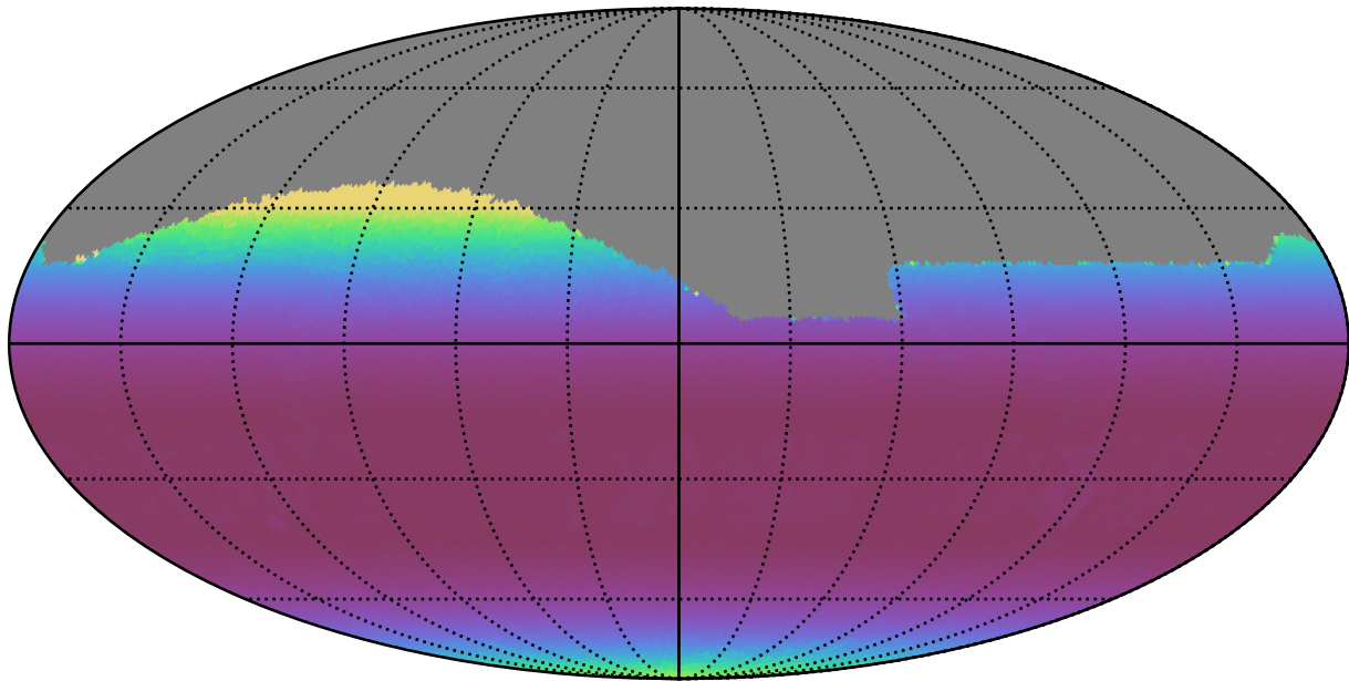
ddf_acor_sf15_lsf40_lsr50_v3.4_10yrs Yr 1 all bands: Min airmass
