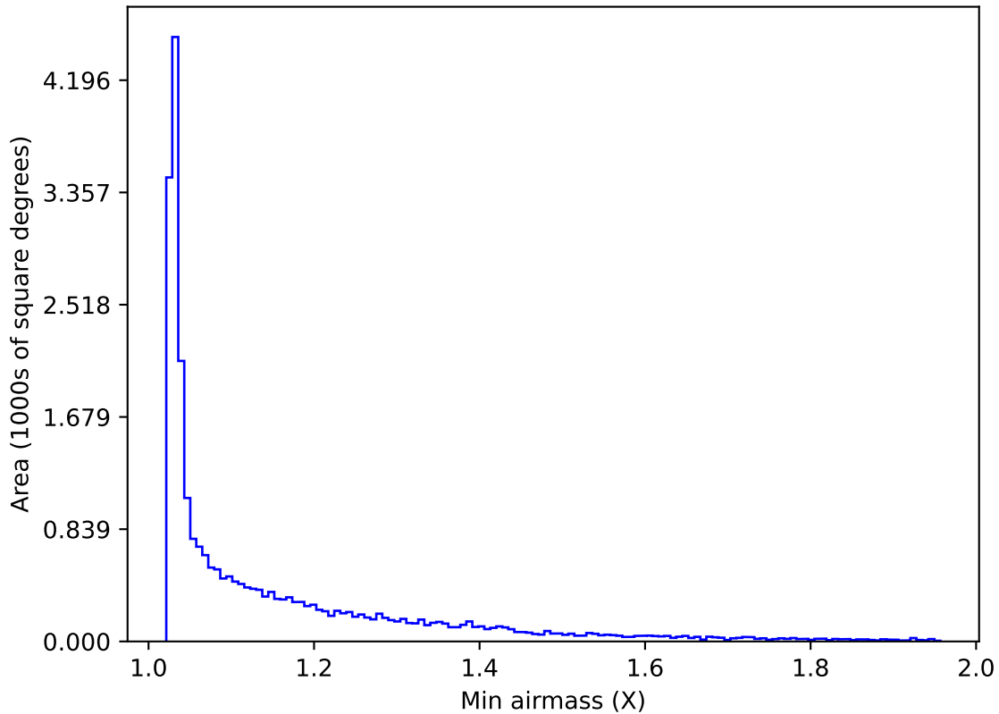
ddf_acor_sf15_lsf40_lsr50_v3.4_10yrs Yr 1 all bands: Min airmass
