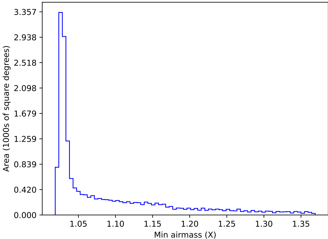
ddf_acor_sf15_lsf40_lsr50_v3.4_10yrs WFD z band: Min airmass
