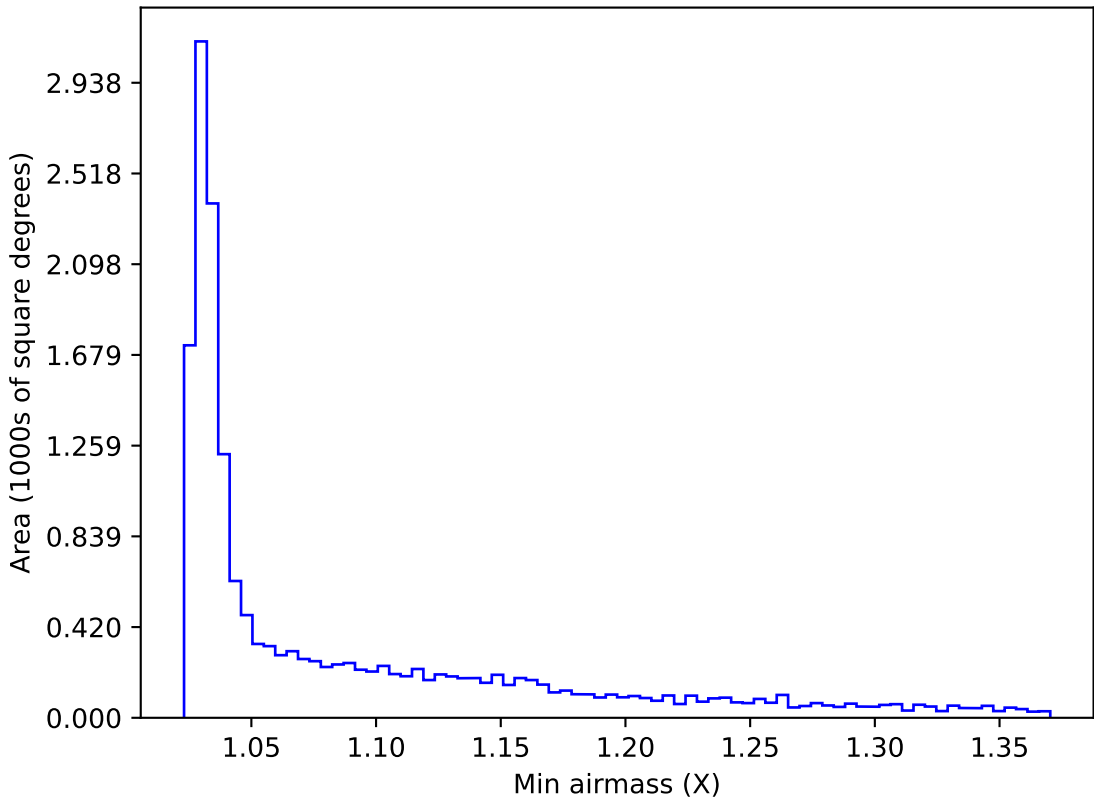
ddf_acor_sf15_lsf40_lsr50_v3.4_10yrs WFD y band: Min airmass
