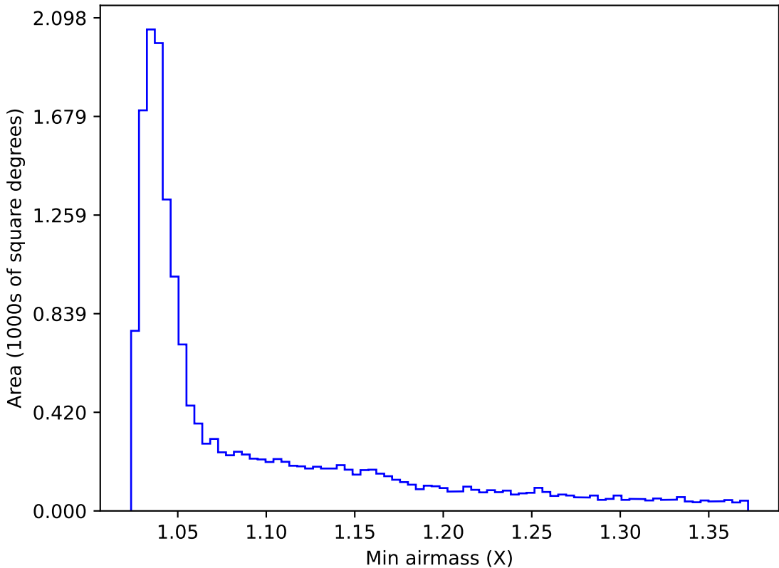
ddf_acor_sf15_lsf40_lsr50_v3.4_10yrs WFD u band: Min airmass
