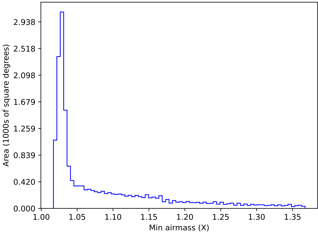
ddf_acor_sf15_lsf40_lsr50_v3.4_10yrs WFD r band: Min airmass
