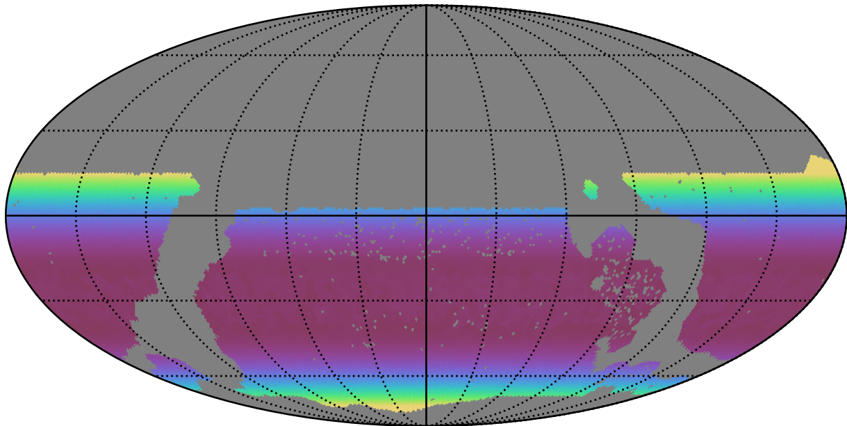
ddf_acor_sf15_lsf40_lsr50_v3.4_10yrs WFD all bands: Min airmass
