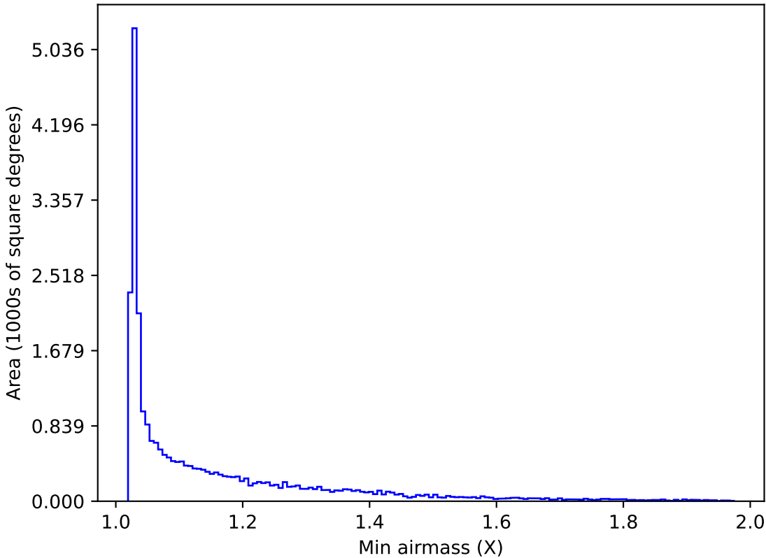
ddf_acor_sf15_lsf40_lsr50_v3.4_10yrs All sky z band: Min airmass
