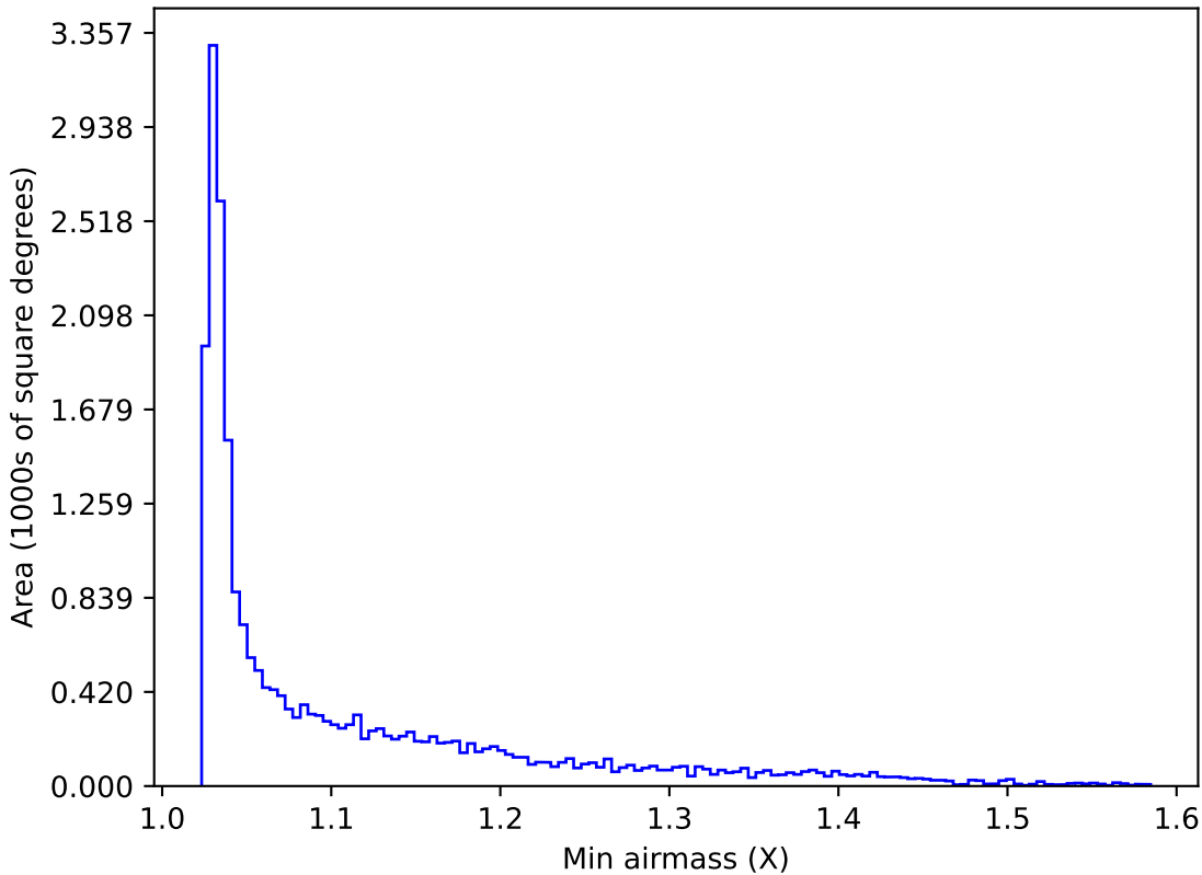
ddf_acor_sf15_lsf40_lsr50_v3.4_10yrs All sky y band: Min airmass
