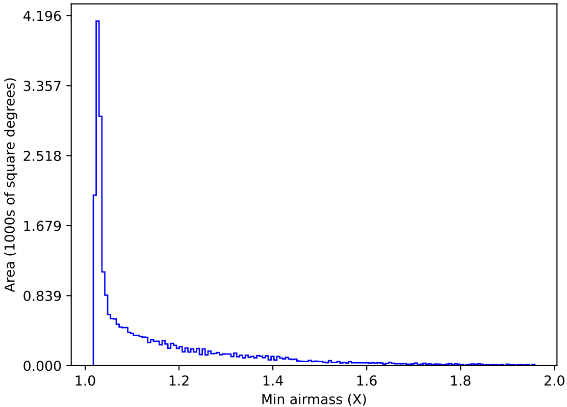
ddf_acor_sf15_lsf40_lsr50_v3.4_10yrs All sky r band: Min airmass
