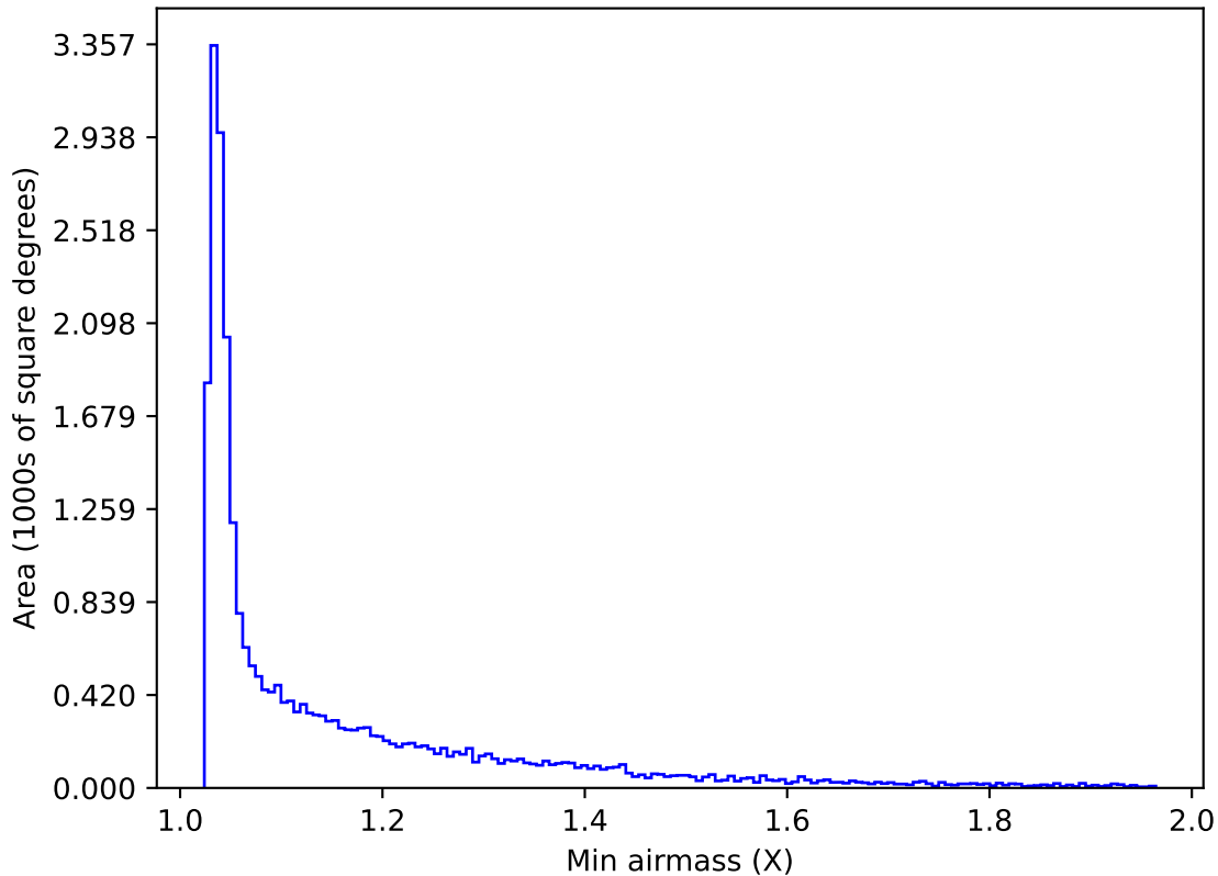
ddf_acor_sf15_lsf40_lsr50_v3.4_10yrs All sky g band: Min airmass
