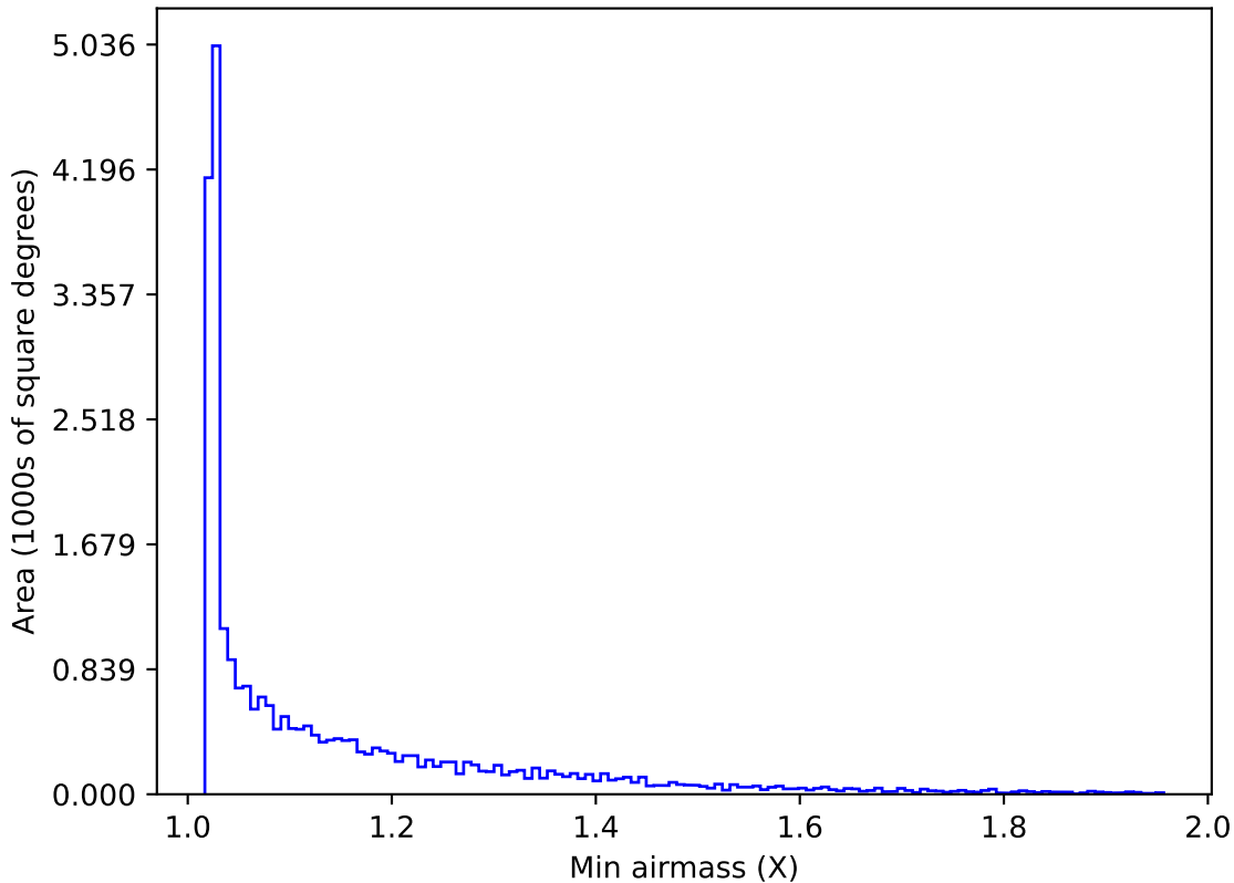
ddf_acor_sf15_lsf40_lsr50_v3.4_10yrs All sky all bands: Min airmass
