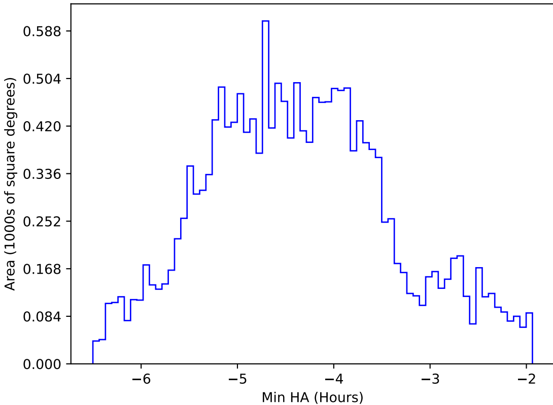
ddf_acor_sf15_lsf40_lsr50_v3.4_10yrs WFD z band: Min HA
