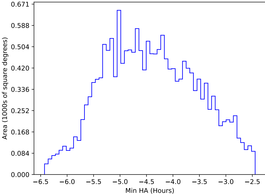
ddf_acor_sf15_lsf40_lsr50_v3.4_10yrs WFD r band: Min HA
