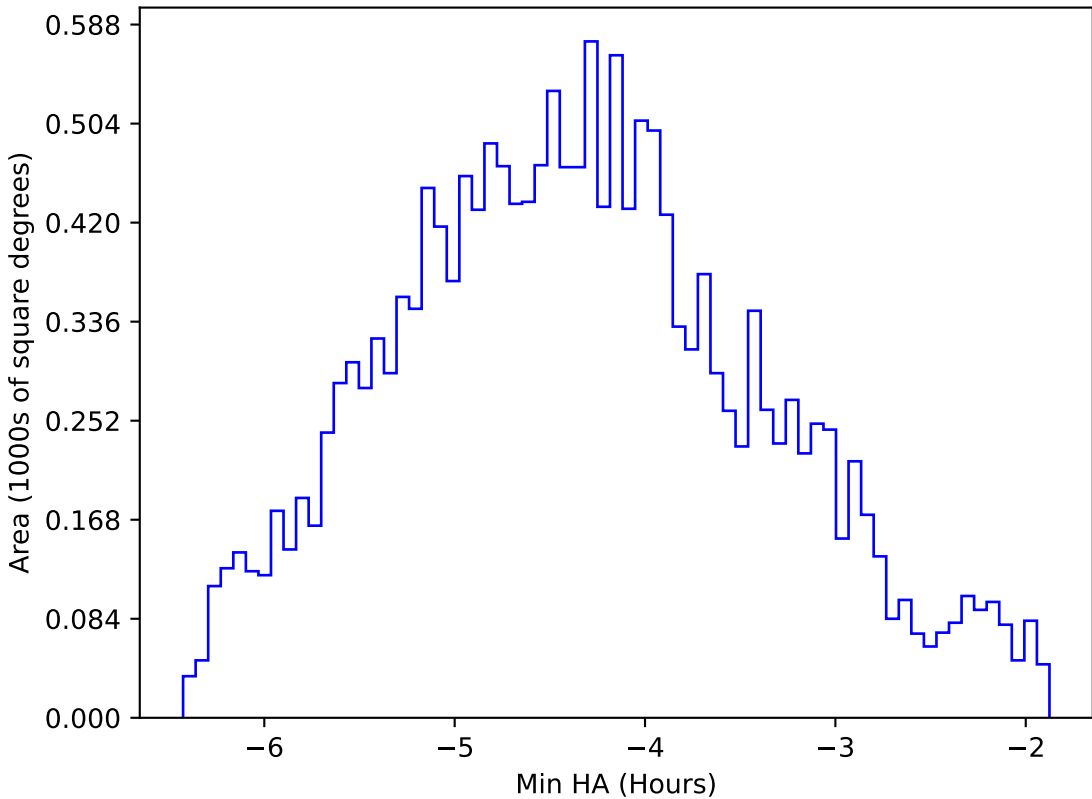
ddf_acor_sf15_lsf40_lsr50_v3.4_10yrs WFD i band: Min HA
