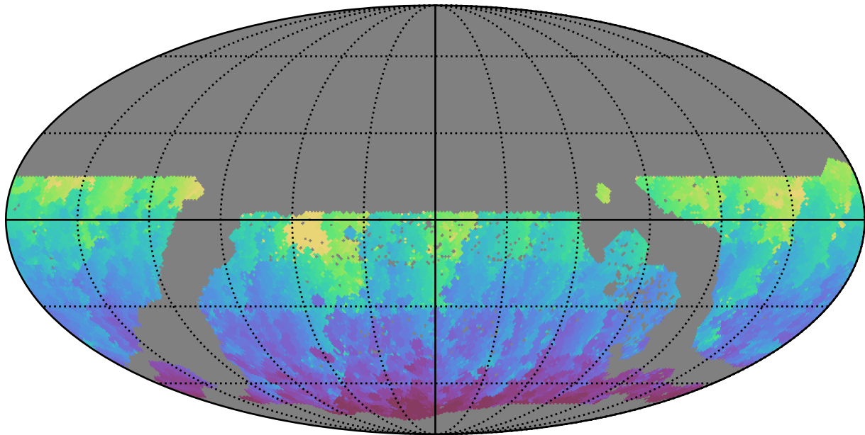
ddf_acor_sf15_lsf40_lsr50_v3.4_10yrs WFD g band: Min HA
